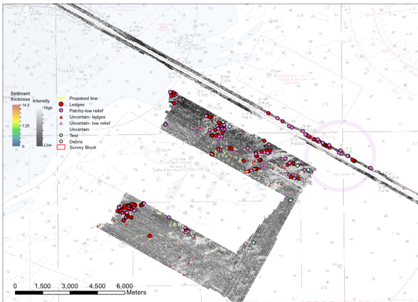
Figure 13. Side scan sonar (backscatter intensity) mosaic overlain with individual targets from full resolution sonar files in Post 45
