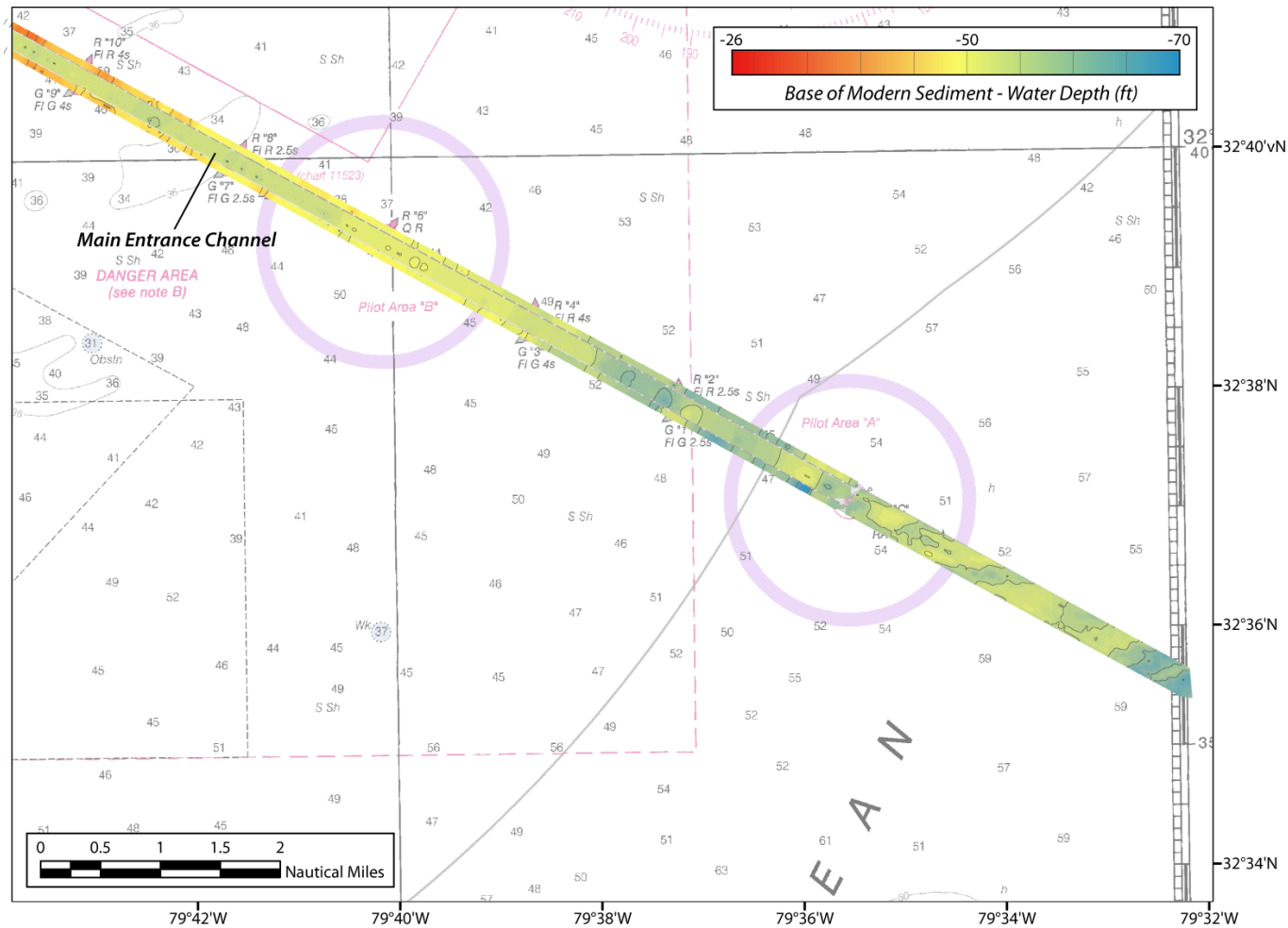
Figure 29. Depth to transgressive surface (base of modern sediment) grid derived from Chirp sub-bottom profiles for the entrance channel extension survey area. Contours are every 5 feet.
