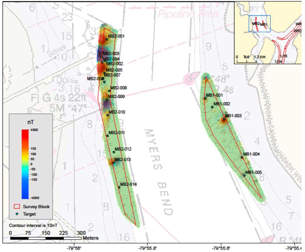
Figure 59. Magnetic anomaly color contour maps of MB1 and MB2.
