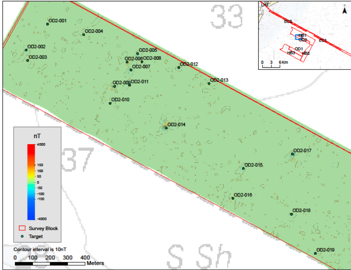
Figure 97. Magnetic anomaly color contour map of OD2.
